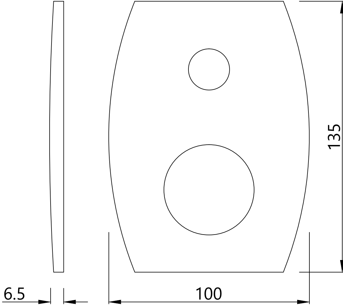
DIVERTER PLATE
