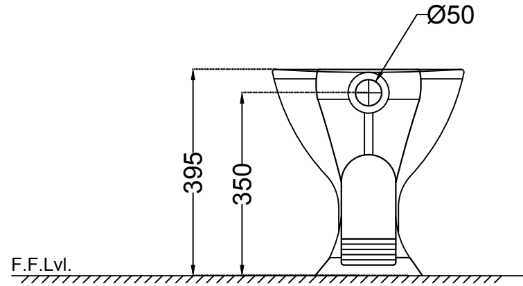
BACK VIEW
